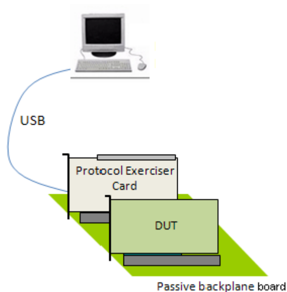
Figure 2 Exerciser Card mounted on a backplane
